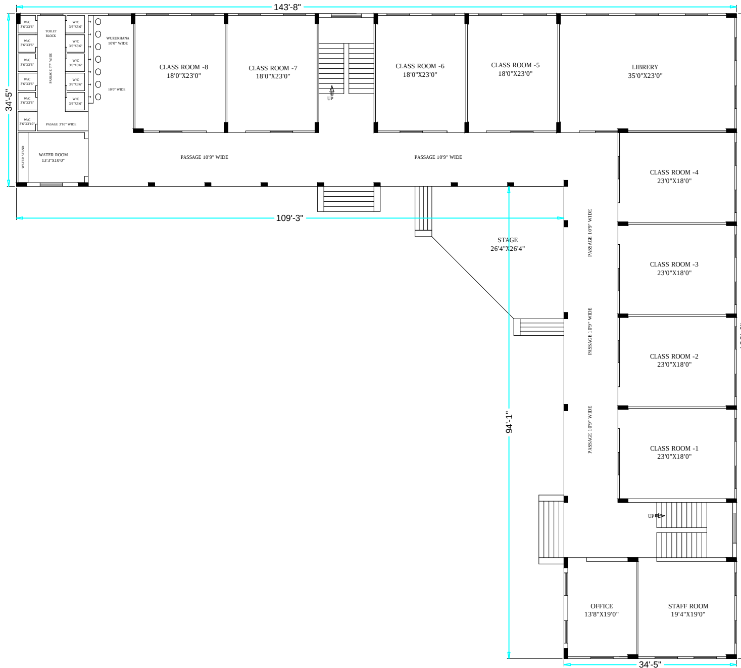
SCHOOL BUILDING TYPICAL FLOOR (G+1)
