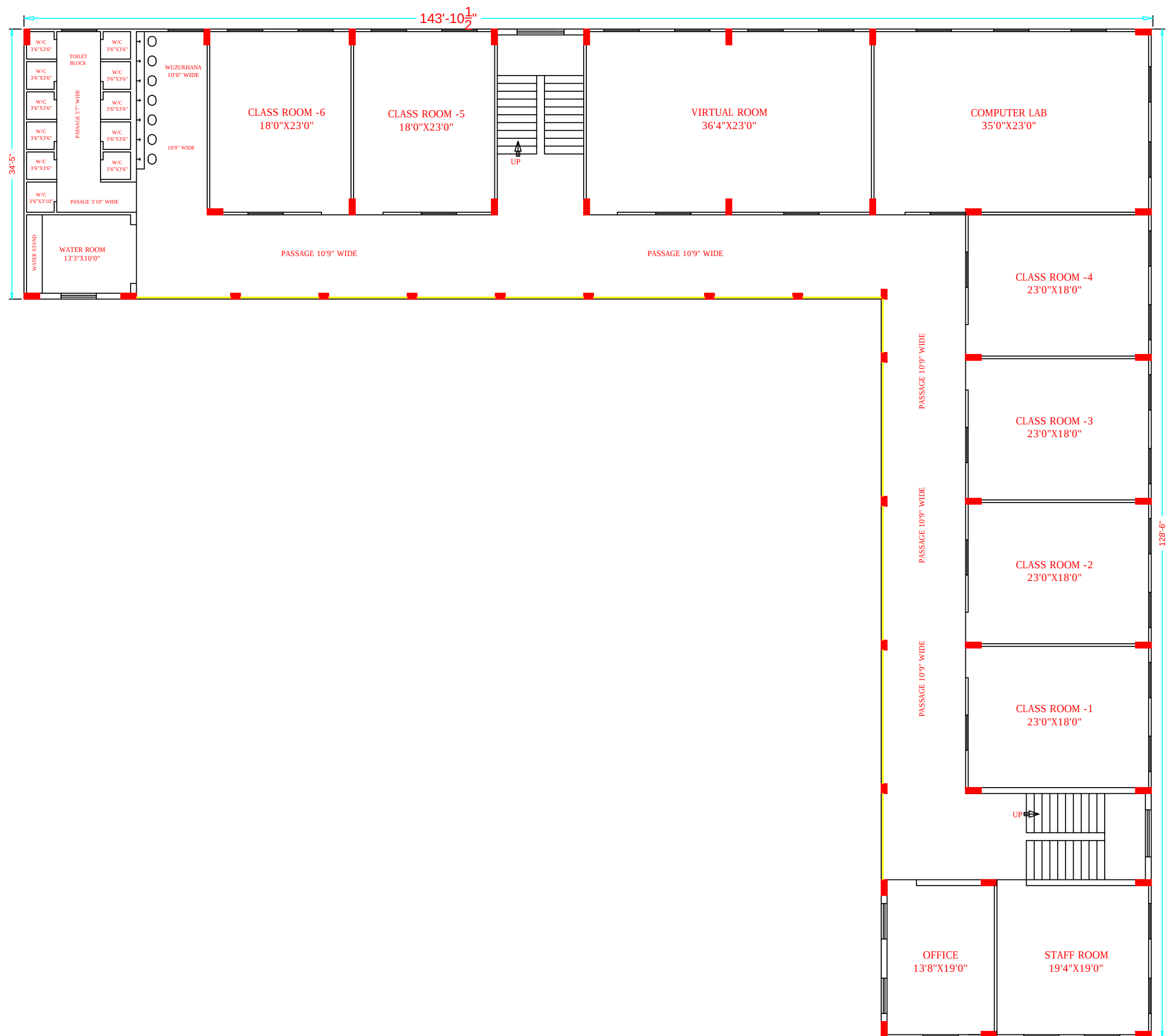
Al Barkaat Girls School ( G+1) FIRST FLOOR
