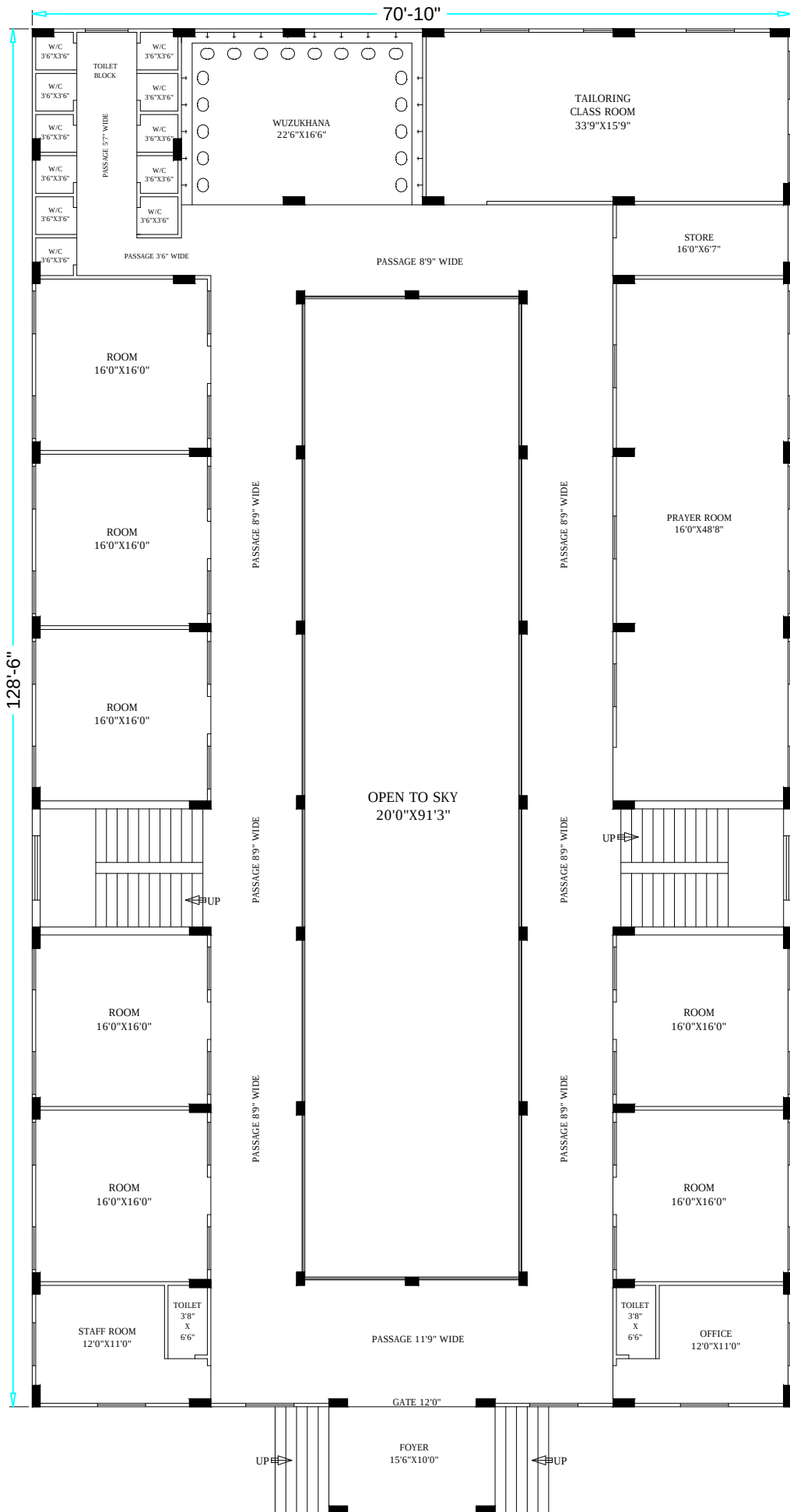
MADRESA BUILDING TYPICAL FLOOR (G+1)
